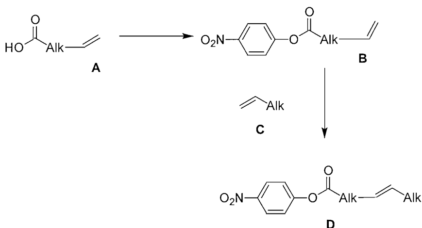
Scheme 1B
