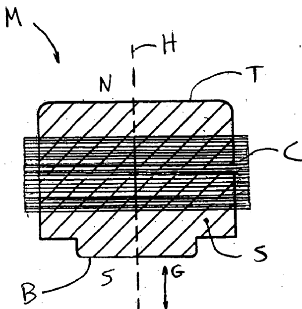
FIG. 4 (PRIOR ART)
