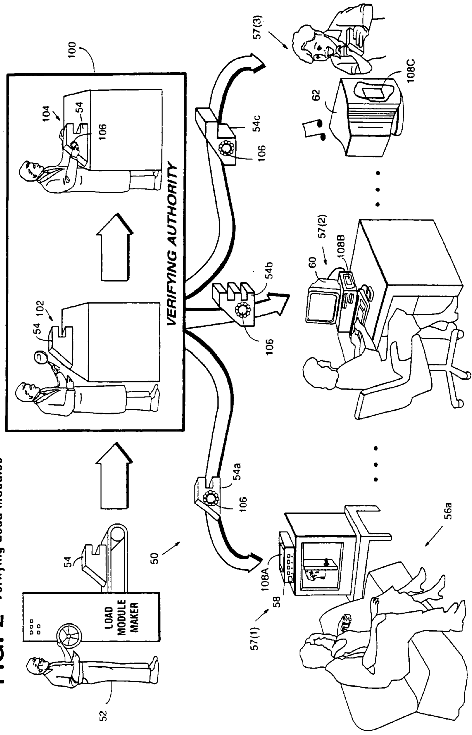
FIG. 2 Verifying Load Modules
