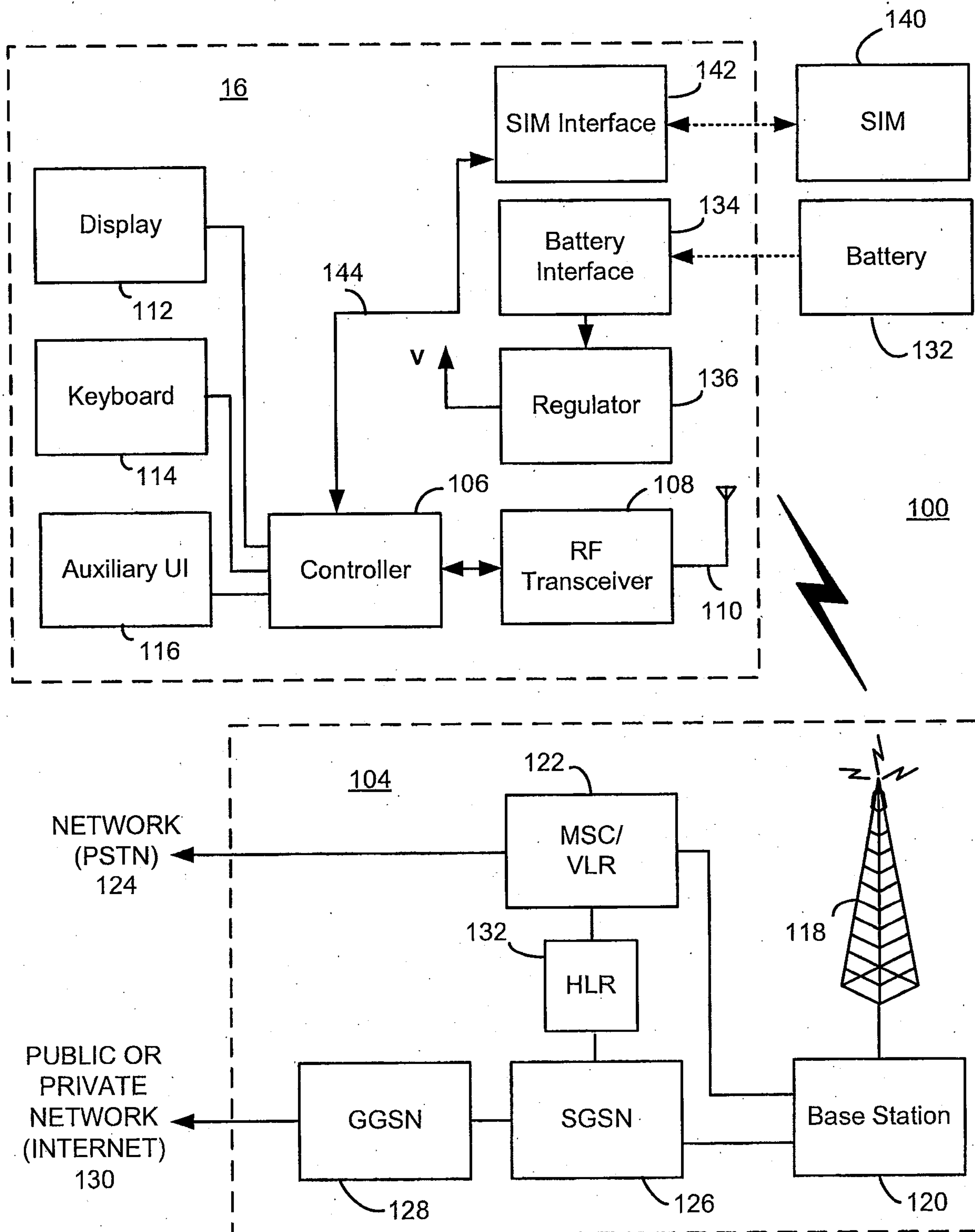
FIG. 5: GPRS Device
