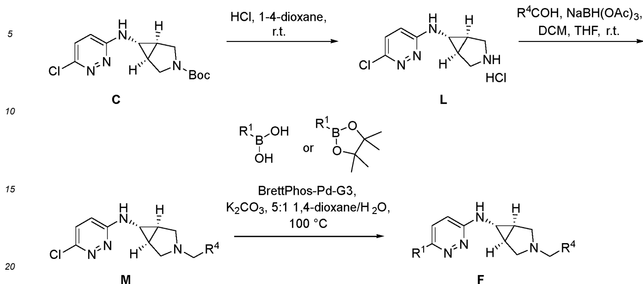
Scheme 3
