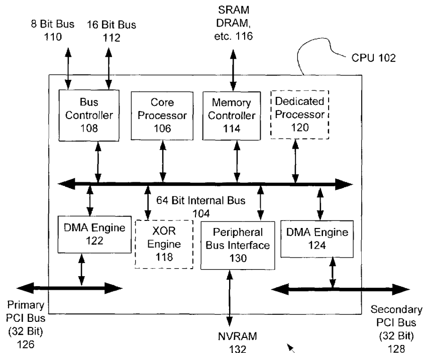
100 Functional Block Diagram of a CPU
