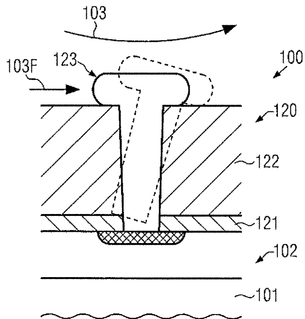
FIG. 1c (prior art)
