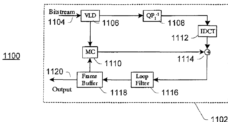
Fig. 11 (Prior Art)
