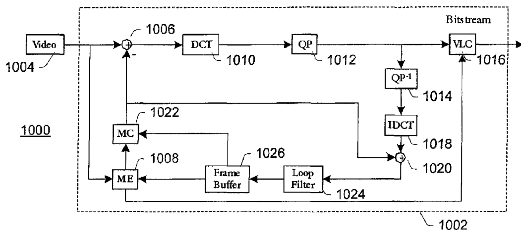
Fig. 10 (Prior Art)
