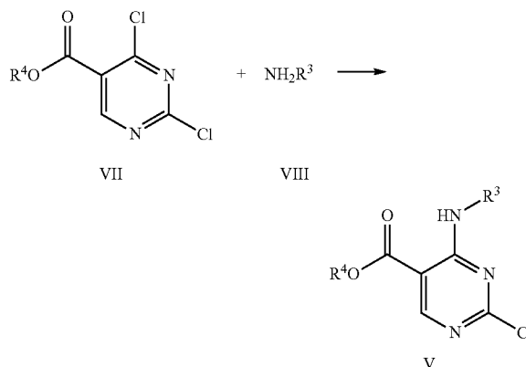
Scheme 4. Coupling of dichloride VII with amine VIII
