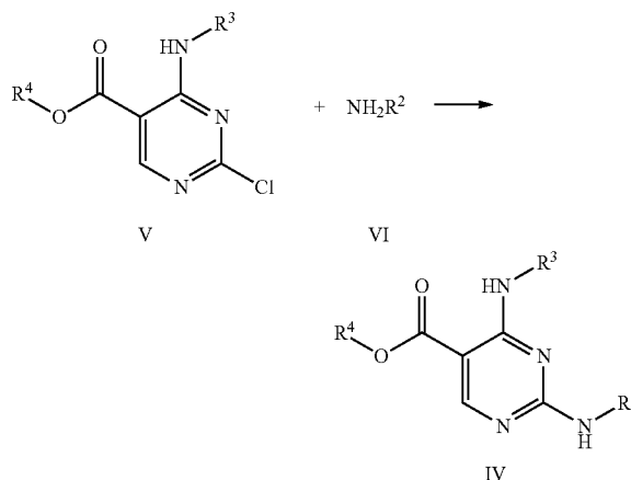
Scheme 3. Coupling of halo-pyrimidine V with amine VI
