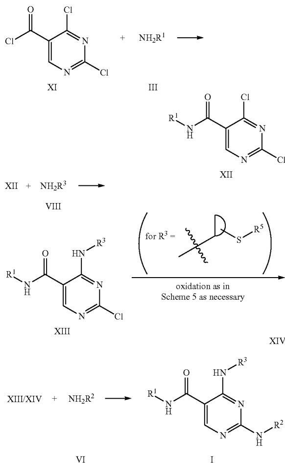
Scheme 6. Synthesis of I from alternate starting material XI
