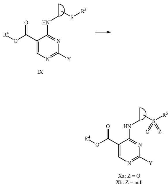
Scheme 5. Oxidation of pendant sulfides IX to Sulfones and Sulfoxides
