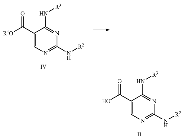
Scheme 2. Saponification of ester IV
