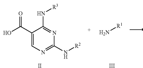
Scheme 1. Coupling of carboxylic acid II with amine III
