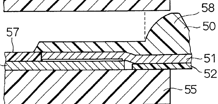
FIG. 8C RELATED ART
