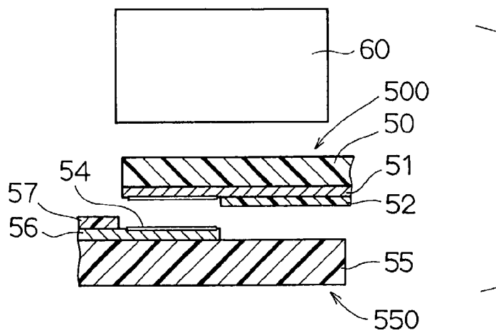
FIG. 7 RELATED ART
