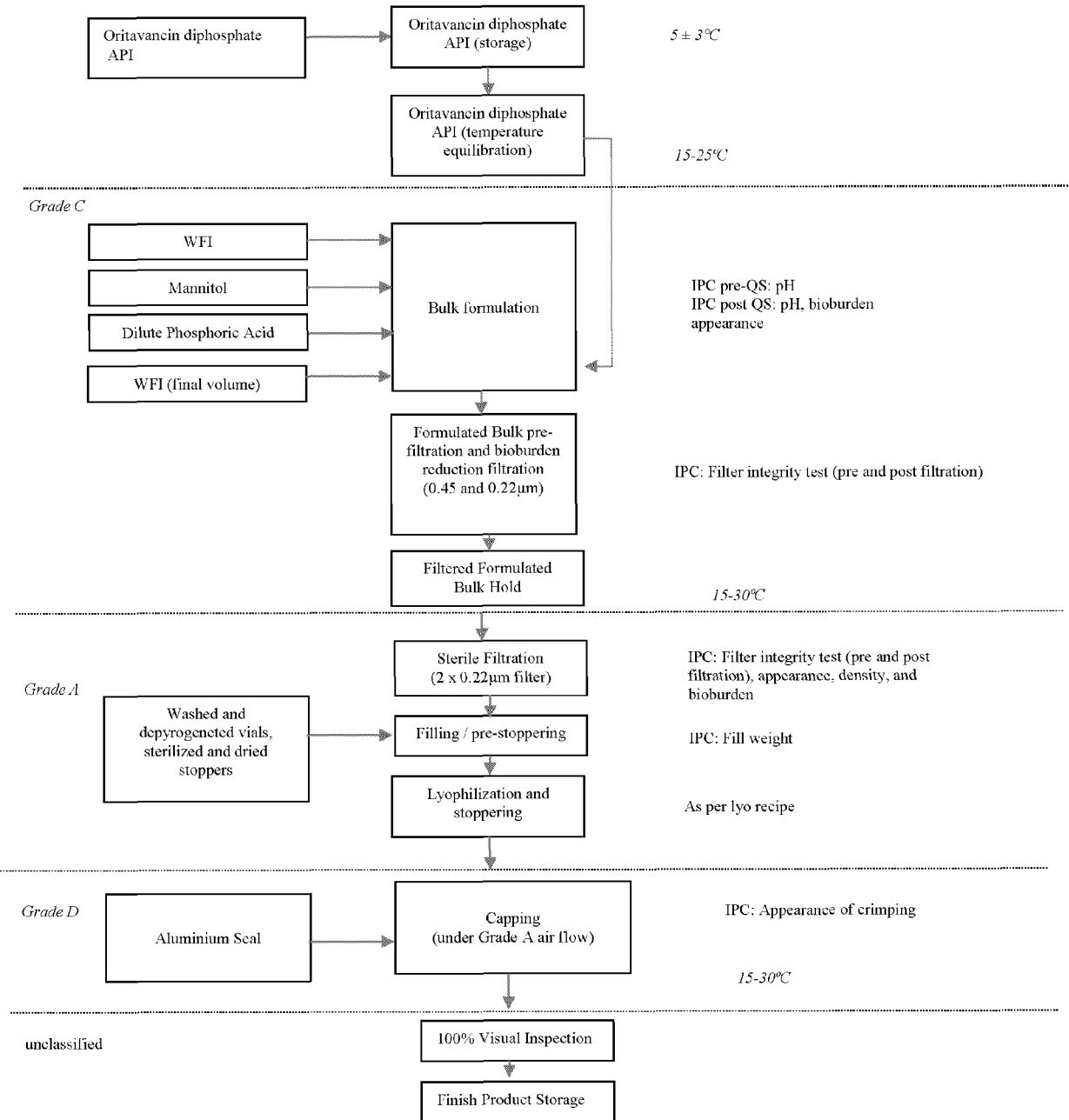
Figure 6 - Schematic Process Flow Diagram of Manufacturing Process
