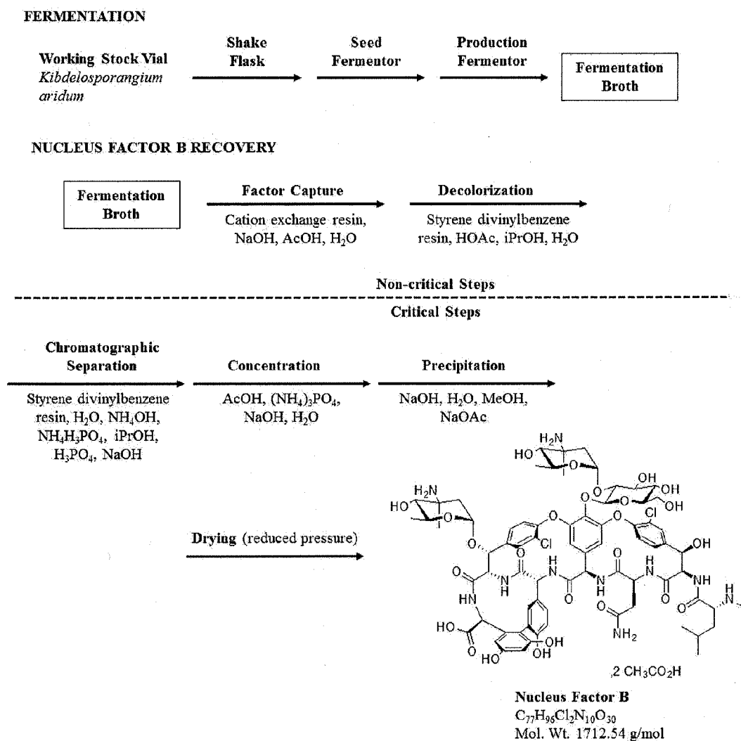
Figure 4 - Nucleus Factor B Diacetate Salt Flow Diagram
