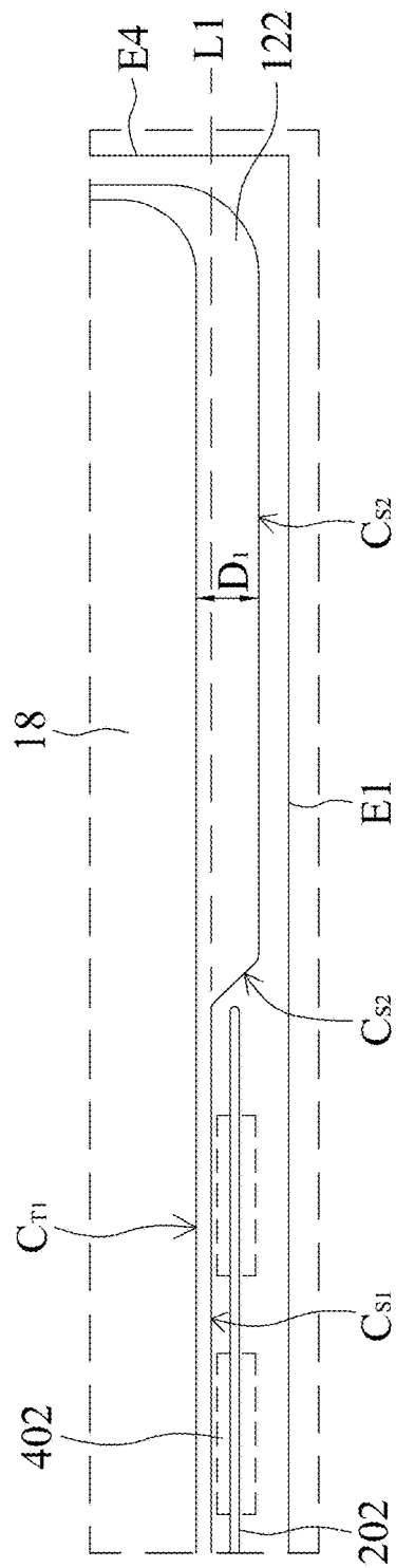
FIG. 2D
