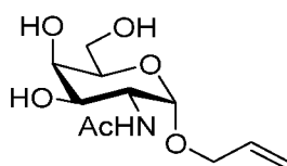
Allyl Tn
