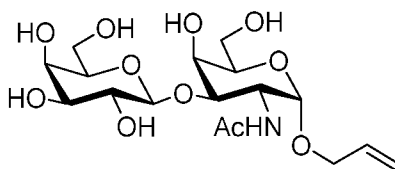
Allyl TF
