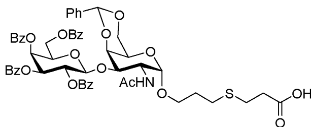
Compound 10
