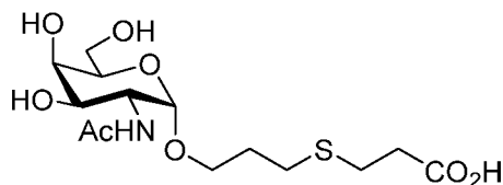
Compound 8
