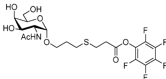
Compound 9
