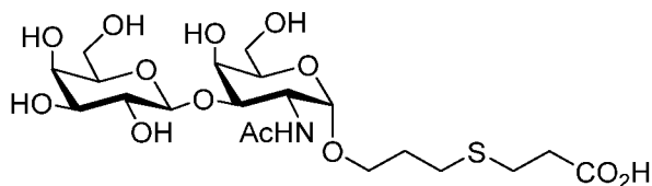
Compound 12
