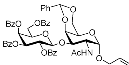
Compound 6
