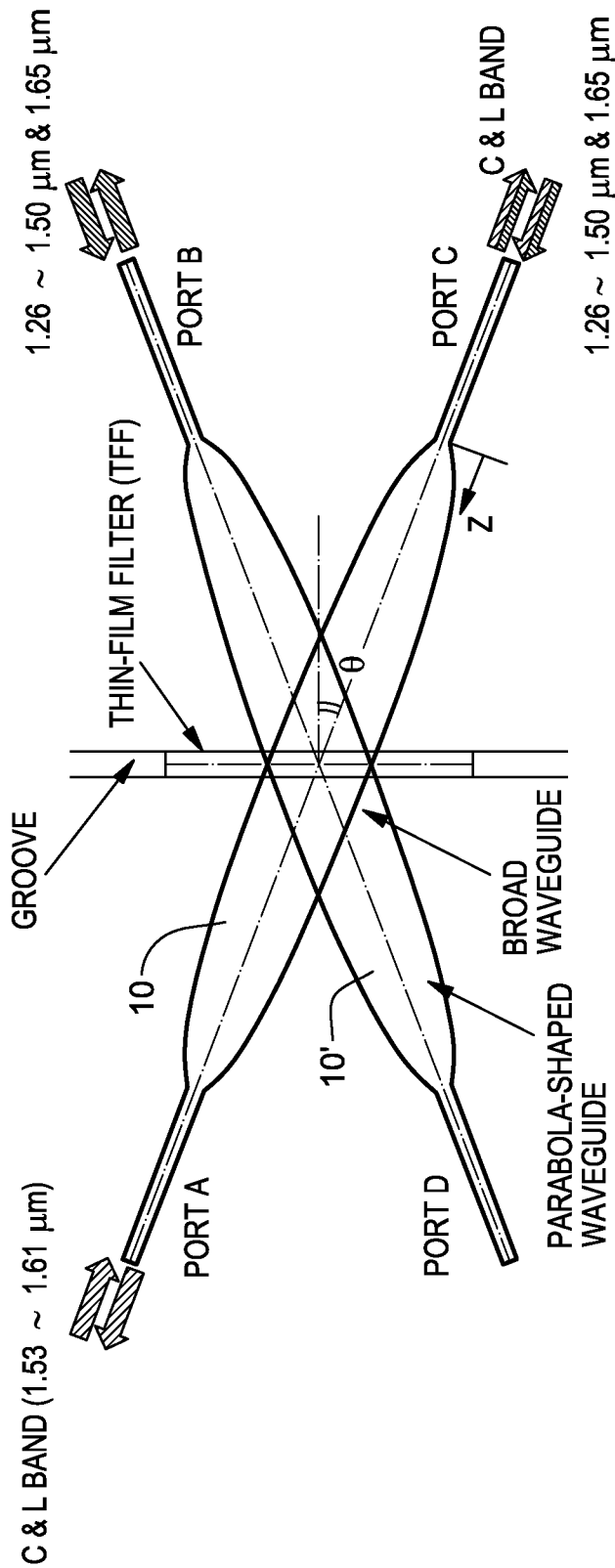
TFF EMBEDDED CROSSING WAVEGUIDES WITH PARABOLA-SHAPED WAVEGUIDE.
