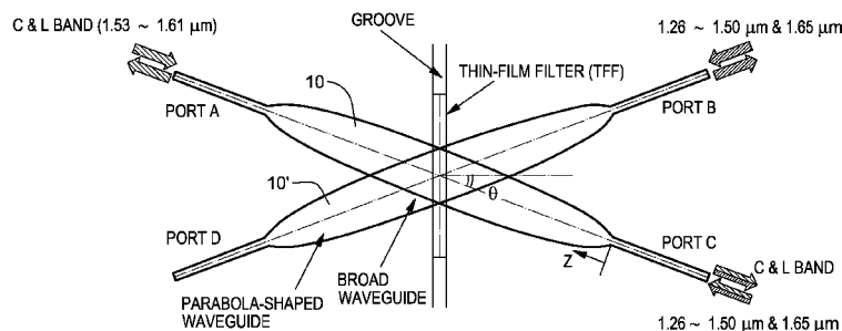
TFF EMBEDDED CROSSING WAVEGUIDES WITH PARABOLA-SHAPED WAVEGUIDE.
