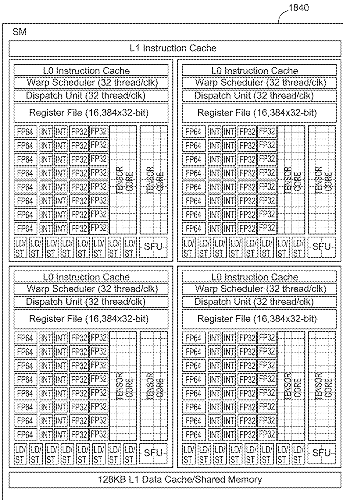
FIG. 22 Example Streaming Multiprocessor
