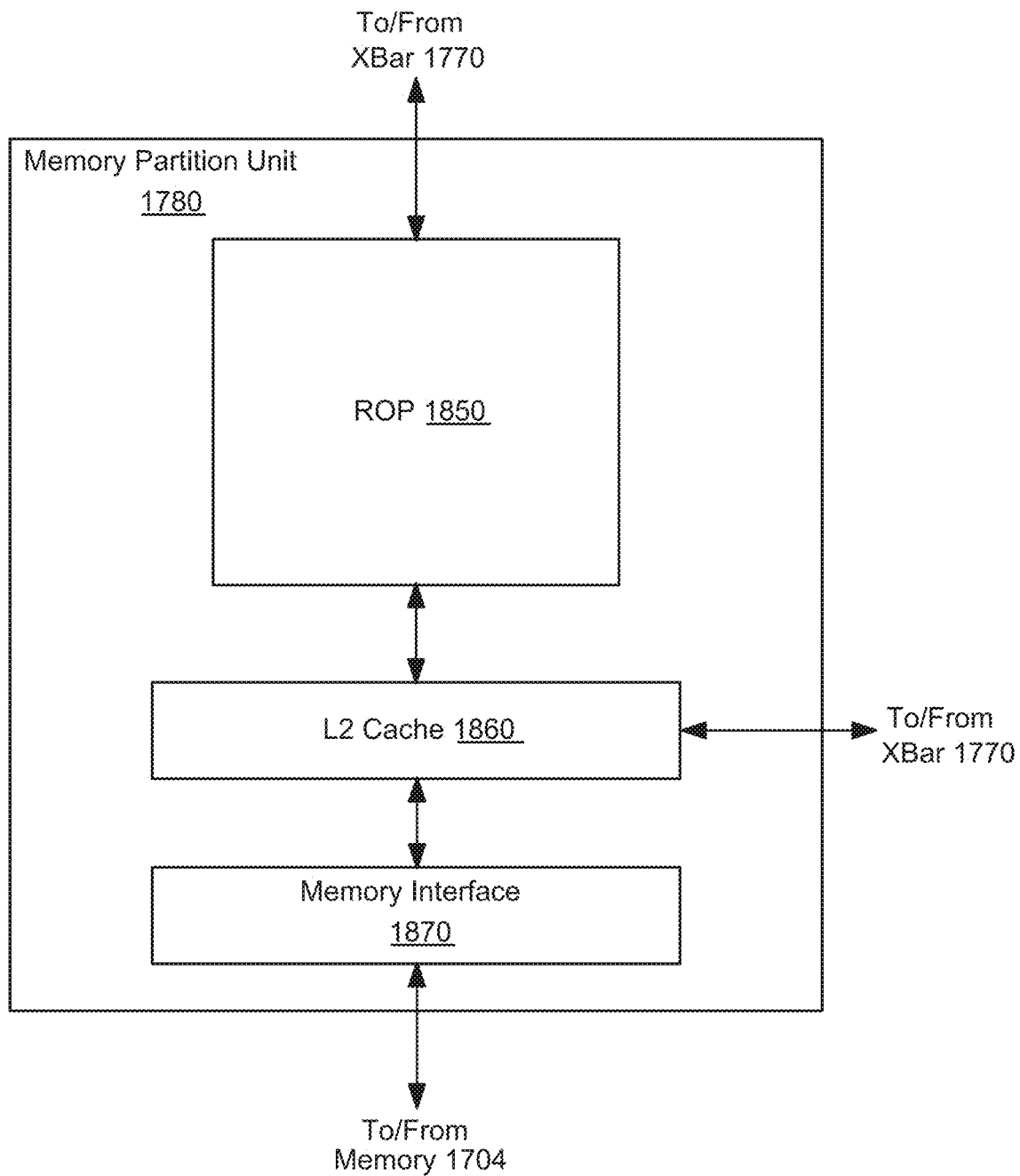
FIG. 18 Example Memory Partition Unit
