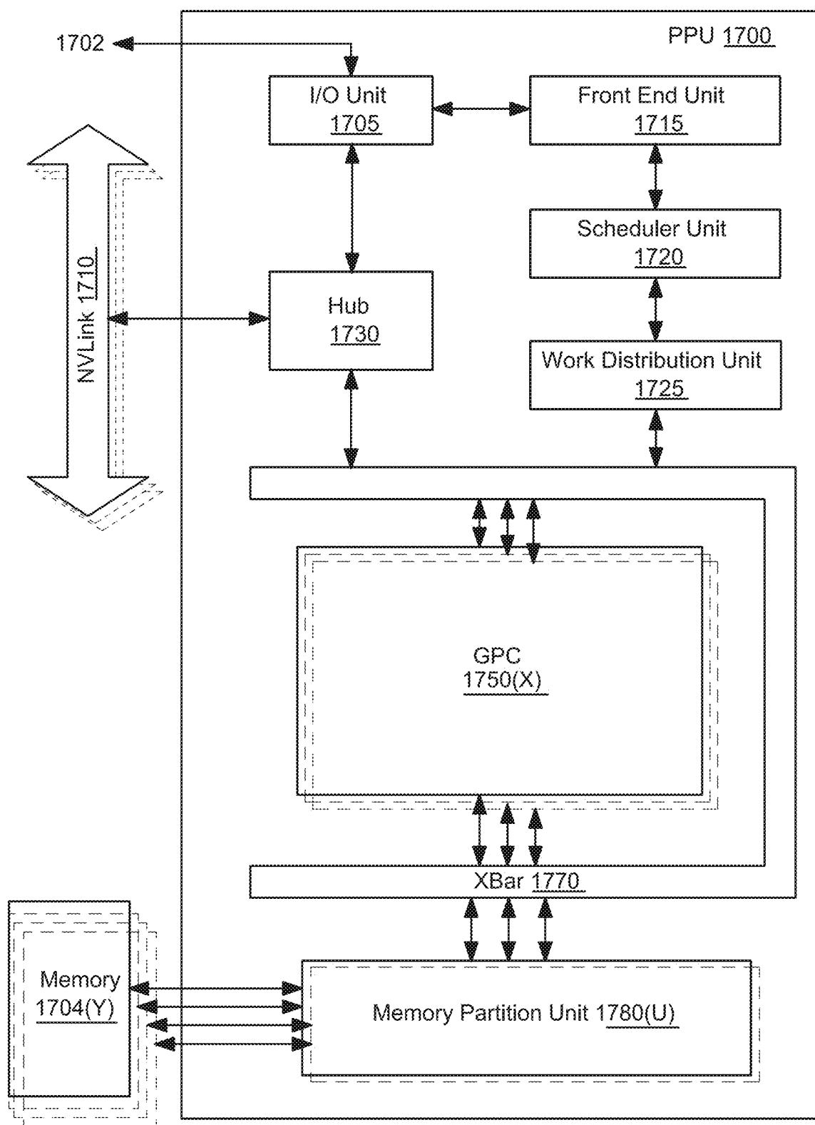
FIG. 17 Example Parallel Processing Unit
