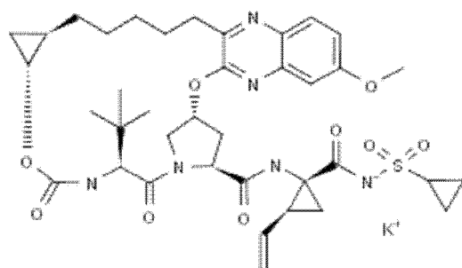
MK-5172
