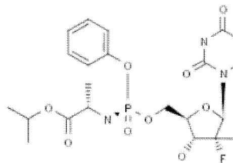
PSI-7977
