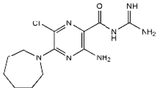
BIT-225
