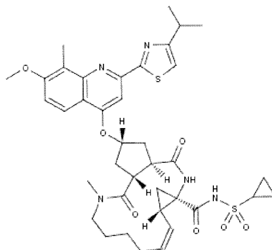
TMC-435 (TMC-435350)
