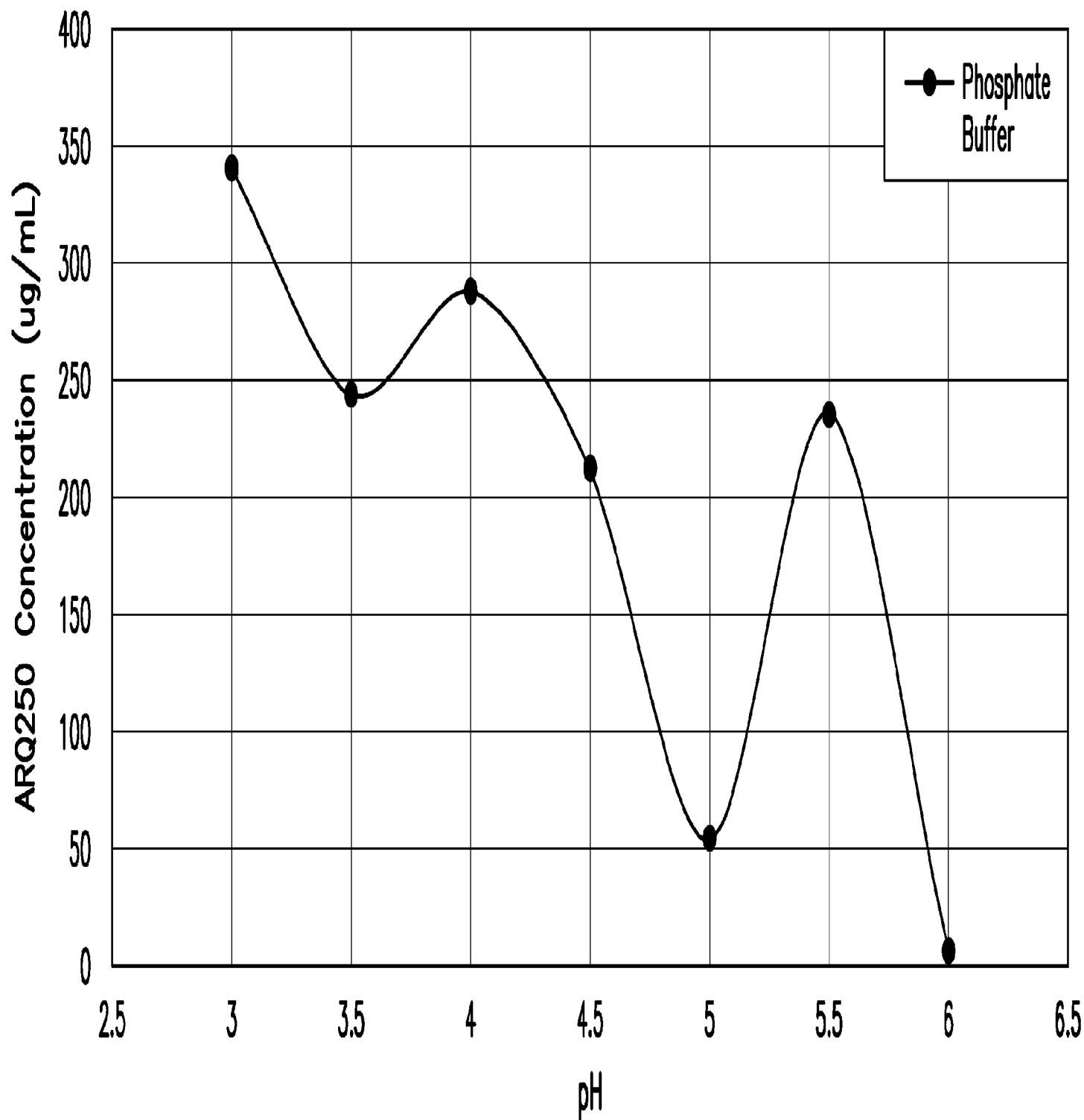
ARQ250 Conc vs. pH in Phosphate Buffer
