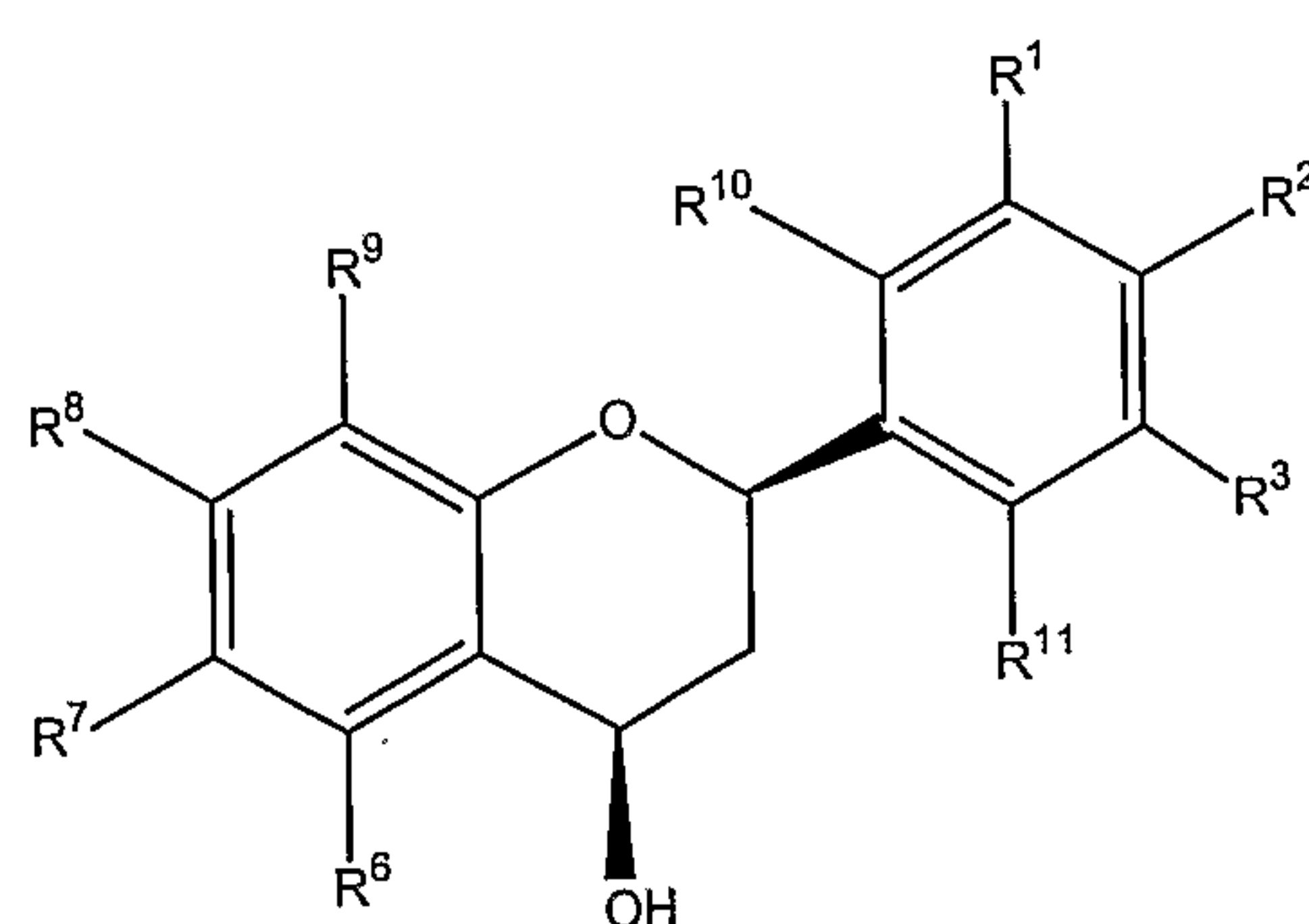
2\alpha,4\alpha - cis (IIIB)
