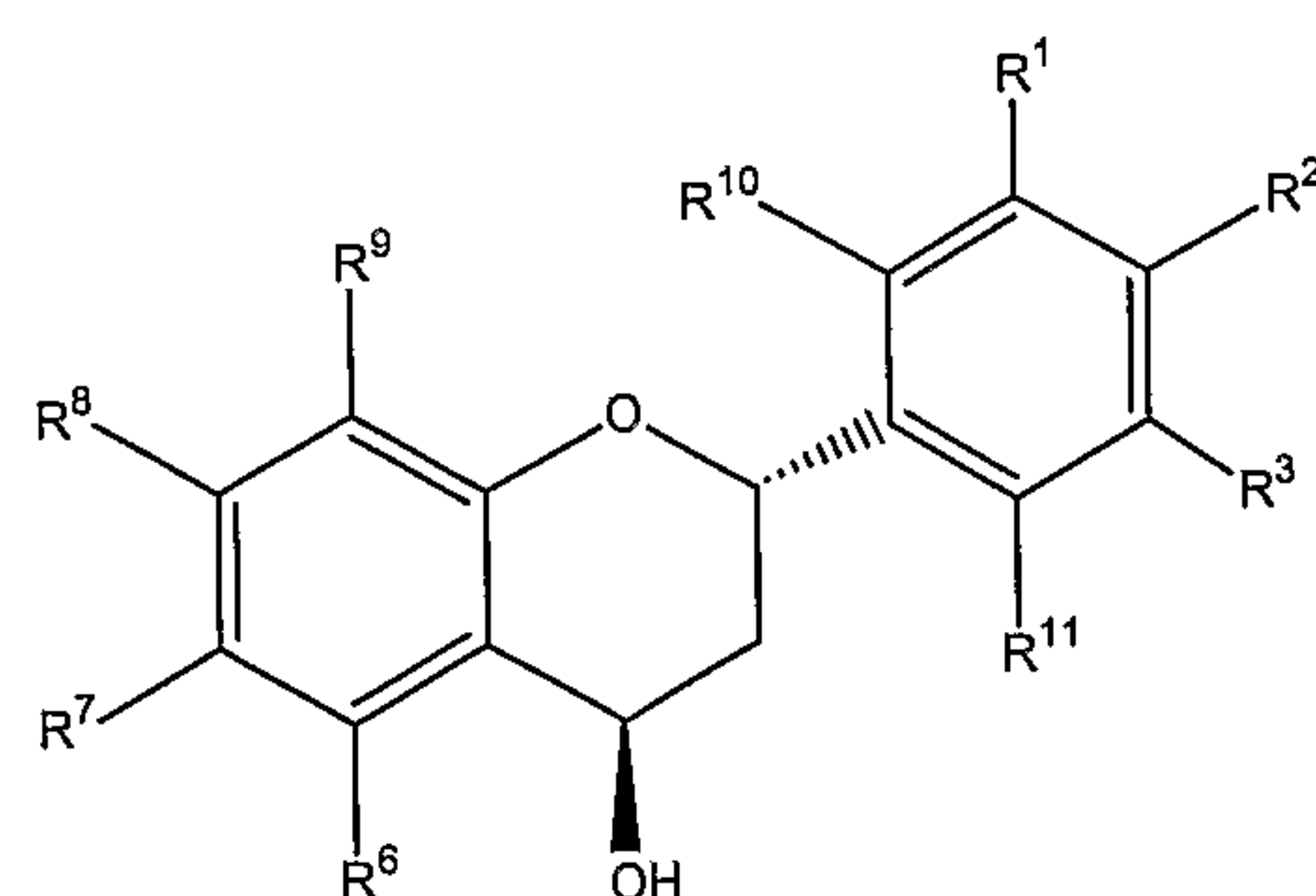
2\alpha,4\alpha - cis (IIIB)
