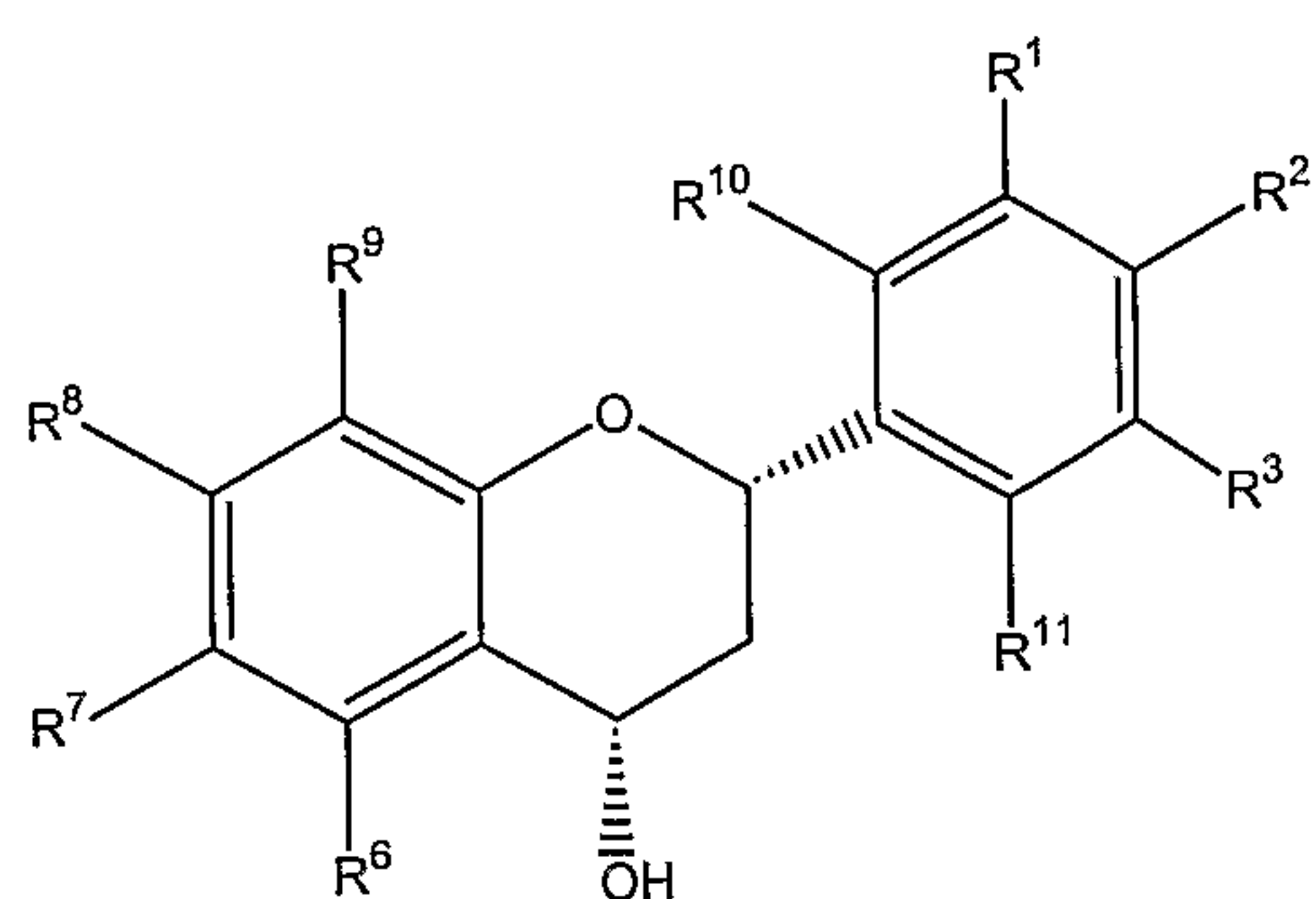
2\beta,4\beta - cis (IIIA)
