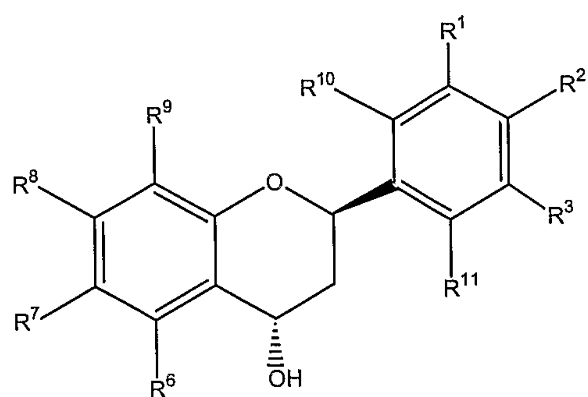
2\alpha,4\beta - trans (IIIC)
