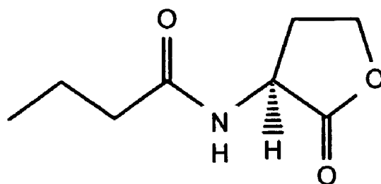
BHL ( N -butanoyl L-homoserine lactone)
