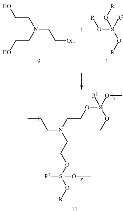
REACTION SCHEME 3
