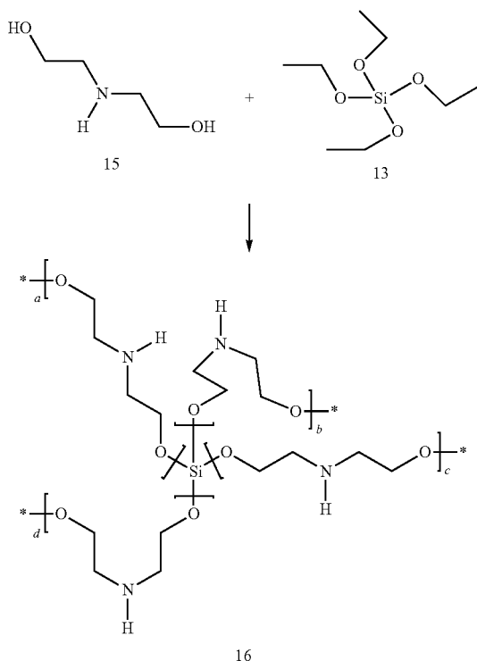
REACTION SCHEME 6
