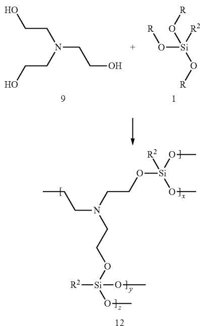
REACTION SCHEME 4
