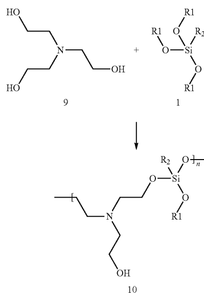
REACTION SCHEME 2
