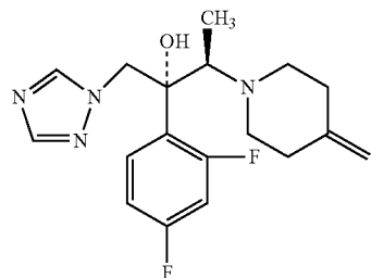
Molecular Formula : \text{C}_{18}\text{H}_{22}\text{F}_2\text{N}_4\text{O} Molecular Weight: 348.39
