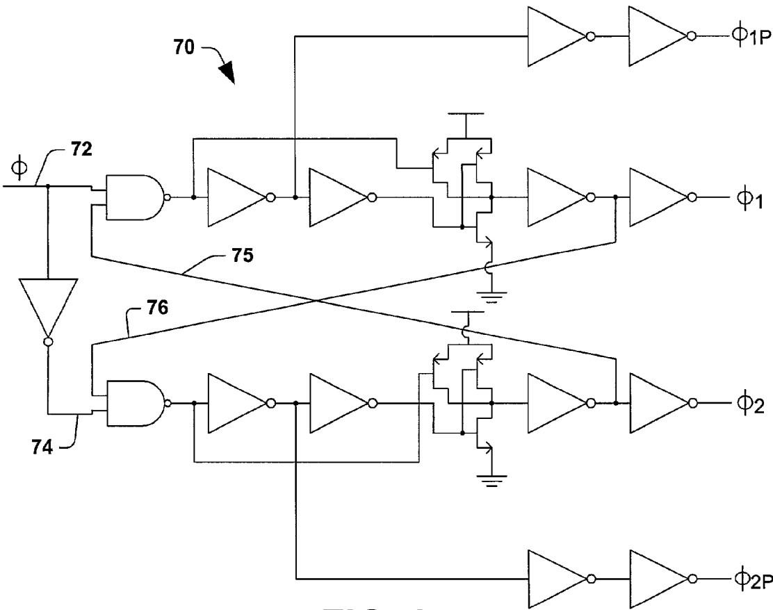
FIG. 6 (PRIOR ART)
