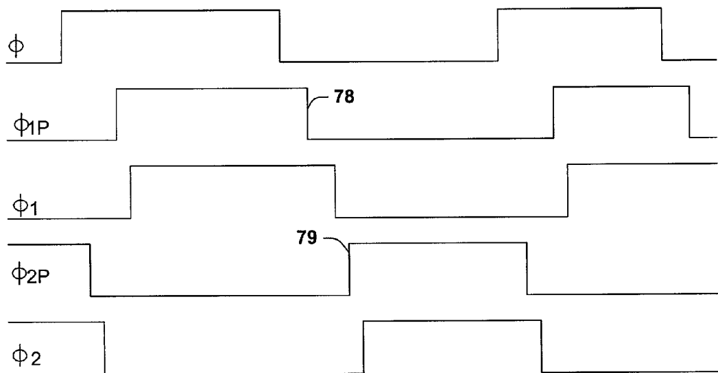
FIG. 7 (PRIOR ART)
