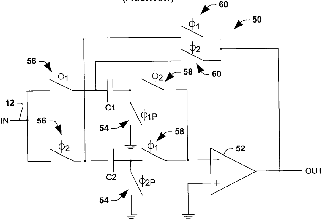
FIG. 4 (PRIOR ART)
