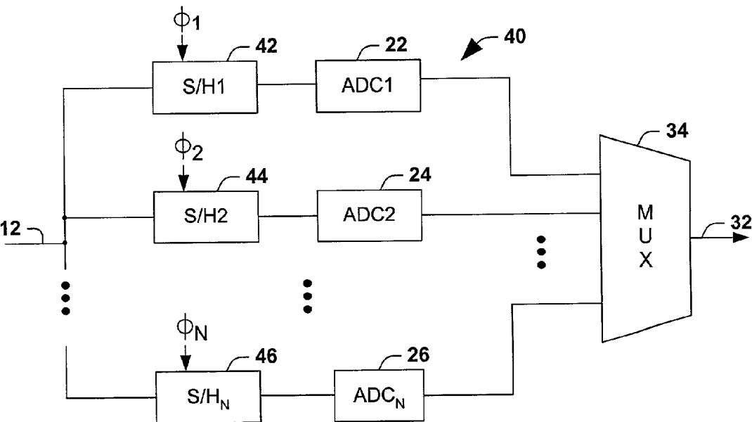
FIG. 3 (PRIOR ART)
