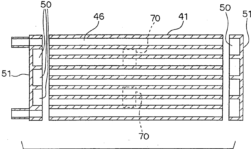
FIG. 47 PRIOR ART
