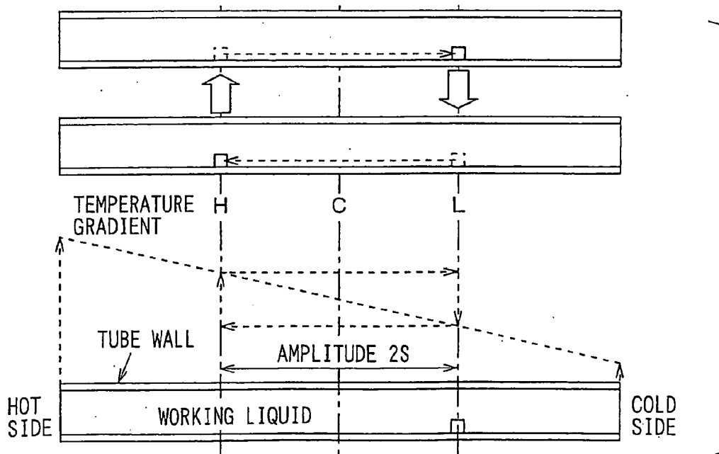
FIG. 22 PRIOR ART
