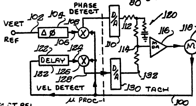
Fig. 7. SCANNER SERVO
