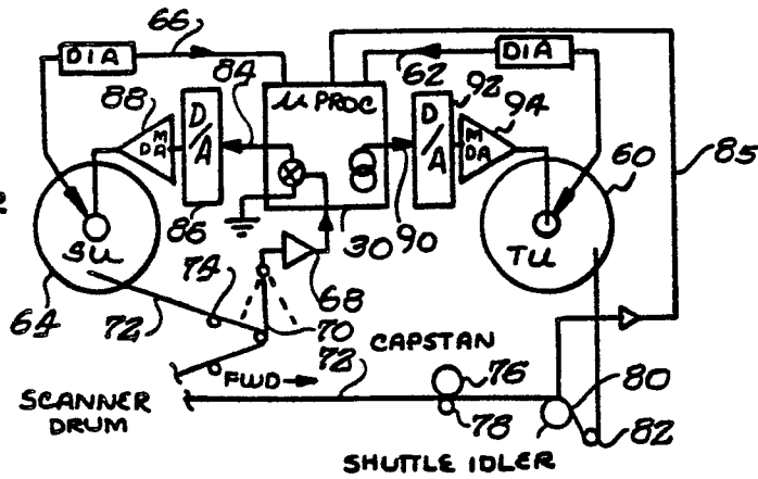
Fig. 5. REEL SERVO REC/PLAY/VAR
