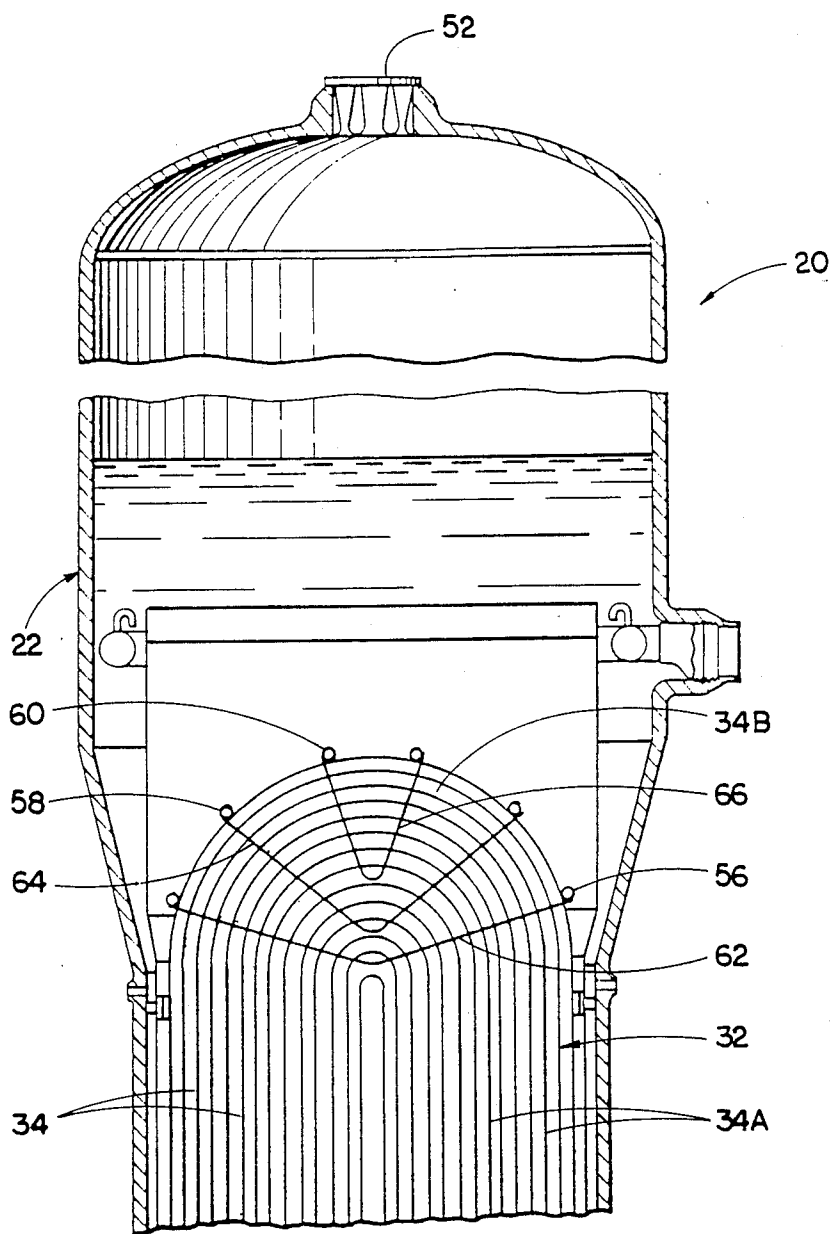
FIG. 2 (PRIOR ART)
