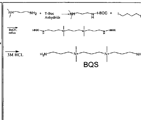
Scheme 2 - BQS linker
