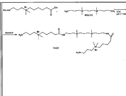
Scheme 4 - TetQS linker
