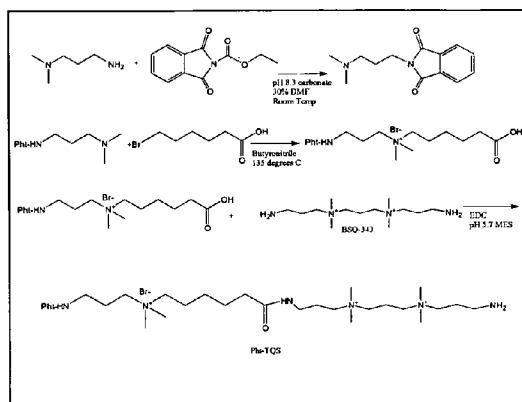
Scheme 3 - TQS linker
