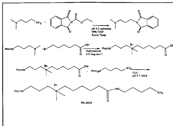
Scheme 1 - MQS component
