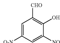
3-Hydroxy-4-Nitrobenzaldehyde (HNBA)
