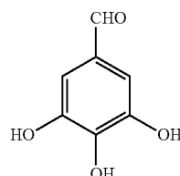
Trihydroxybenzaldehyde (THB-CHO)
