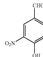
4-Hydroxy-3-Nitrobenzaldehyde (NHBA)
