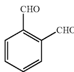
Phthalaldehyde
