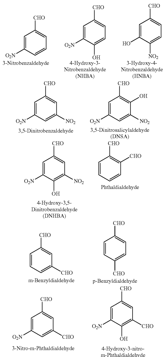
Scheme 2:
