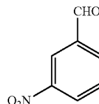
3-Nitrobenzaldehyde
