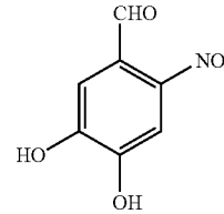
3,4-Dihydroxy-6-nitrobenzaldehyde (DH6NB)
