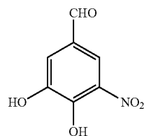
3,4-Dihydroxy-5-nitrobenzaldehyde (DHNB)
