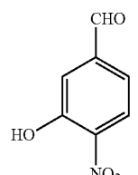
3-Hydroxy-4-Nitrobenzaldehyde (HNBA)
