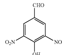
4-Hydroxy-3,5-Dinitrobenzaldehyde (DNHBA)
