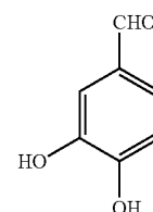
3,4-Dihydroxybenzaldehyde (DHB-CHO)
