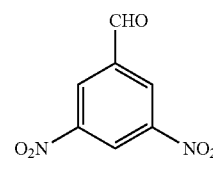
3,5-Dinitrobenzaldehyde
