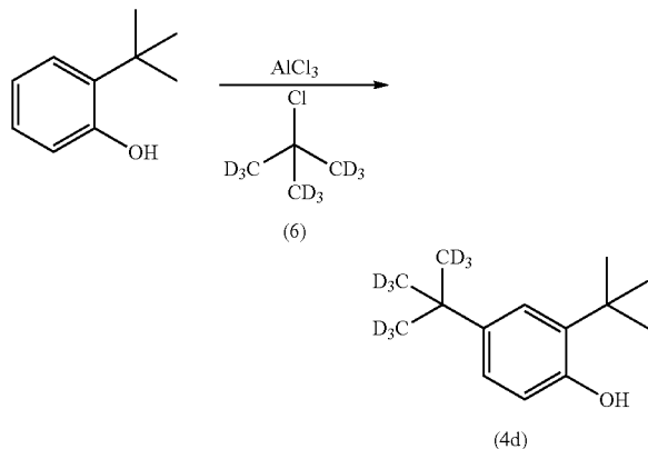
Scheme 4d:
