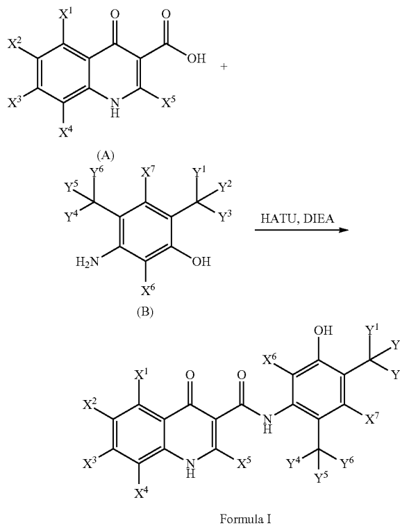
Formula I
