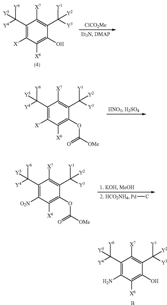
Scheme 3:
