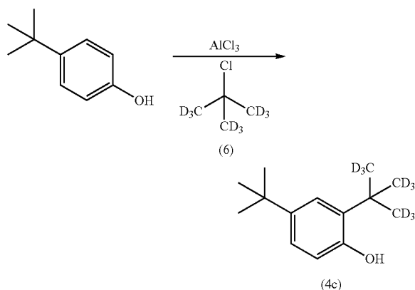
Scheme 4c:
