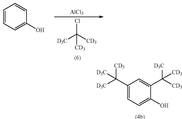
Scheme 4b:
