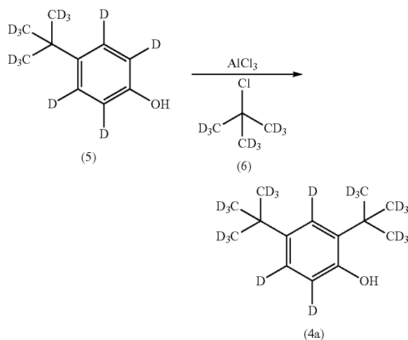
Scheme 4a:
