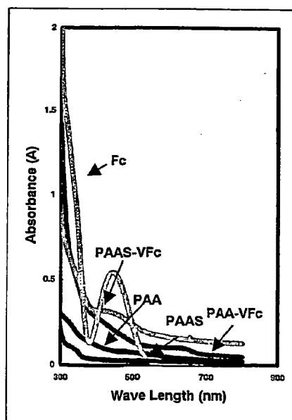
UV-visible spectra of Fc, PAA, PAAS and their VFc co-polymers.
