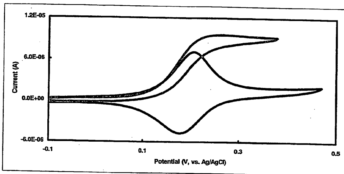
Cyclic voltammogram of cross-linked PAA-VFc-GOx-BSA film on gold electrode. PBS, potential scan rate 50 mV/s
