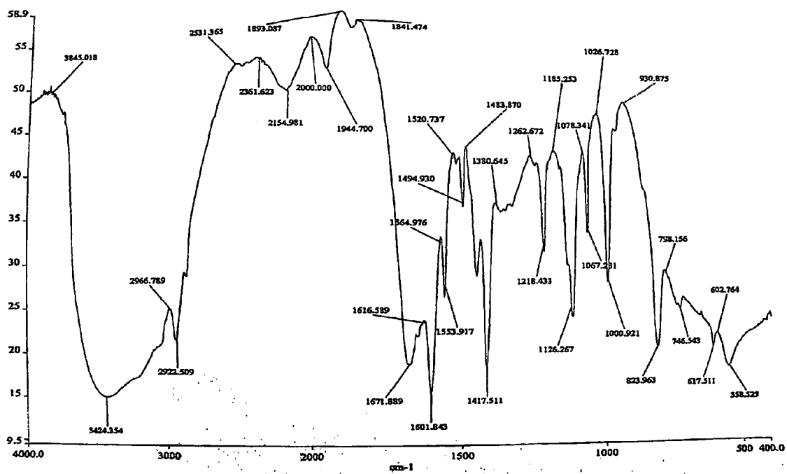
FT-IR Spectrum of PAA-VFc and PAAS-VFc redox polymer
