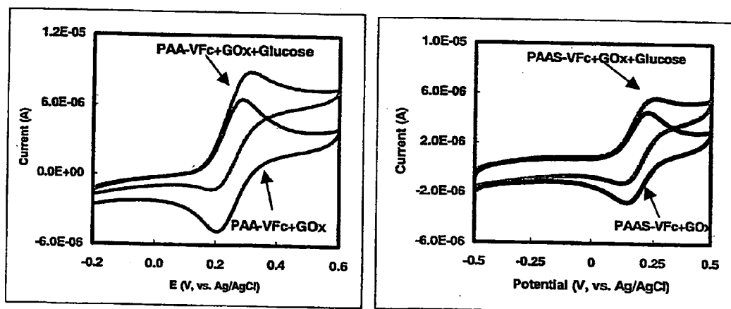
Cyclic voltammograms of redox polymers in various systems.
