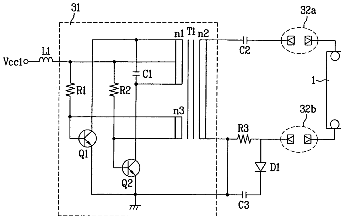
FIG. 4 Related Art
