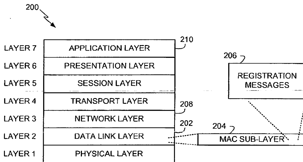
COMMUNICATION LAYER ARCHITECTURE FIG. 2
