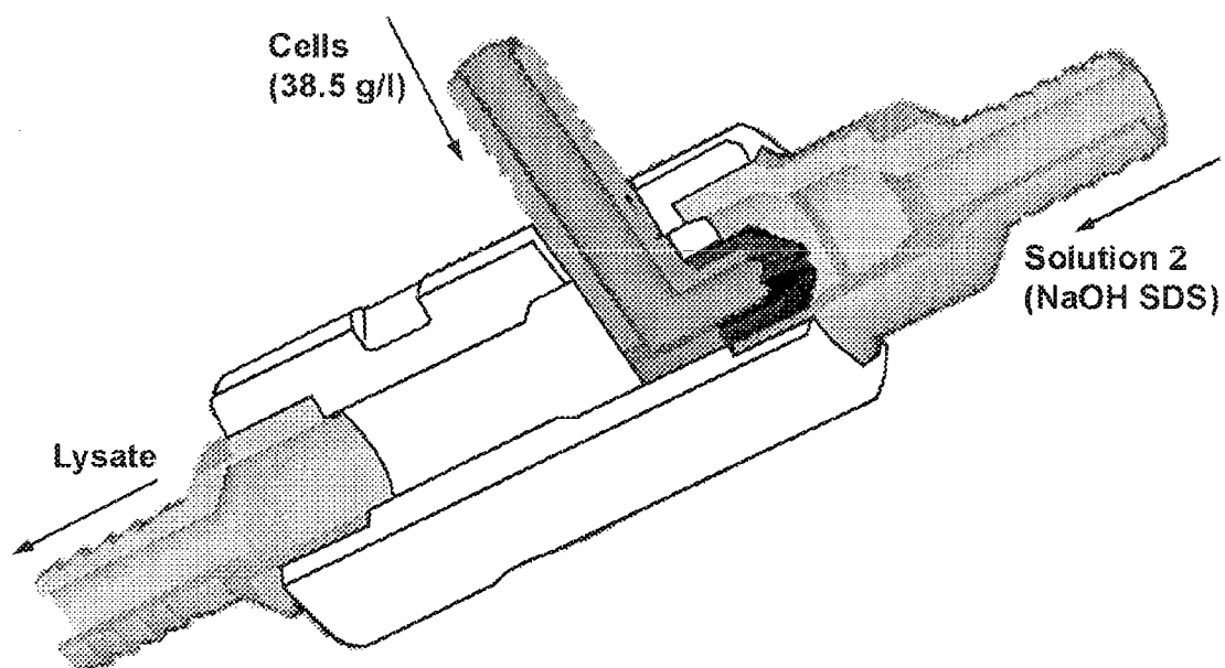
General view of mixer M1
