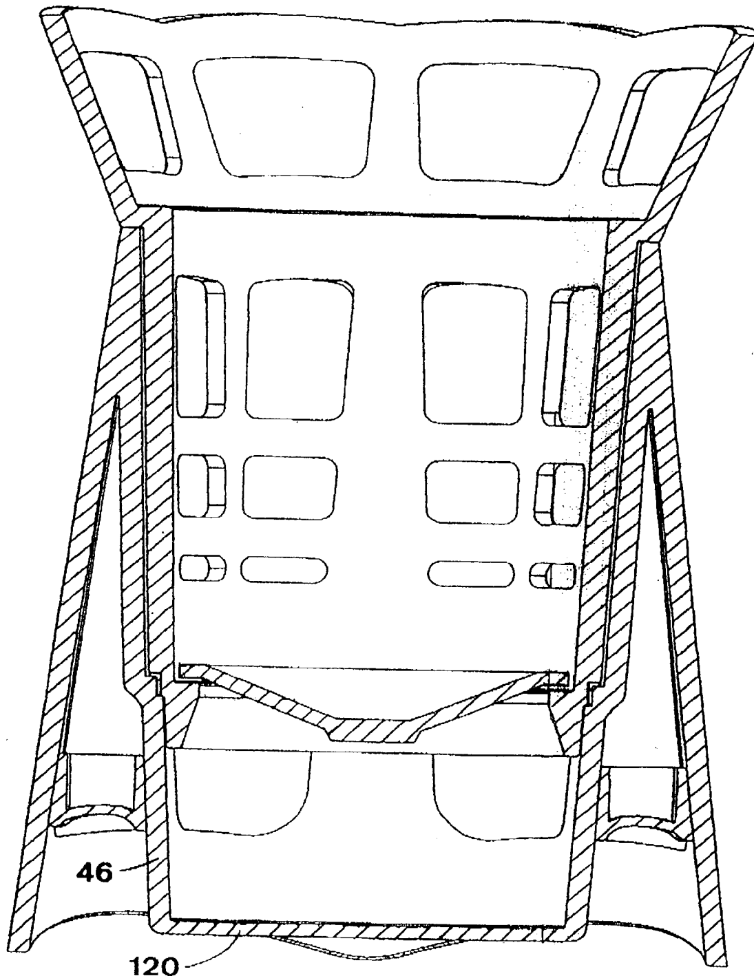
SECTION B-B
