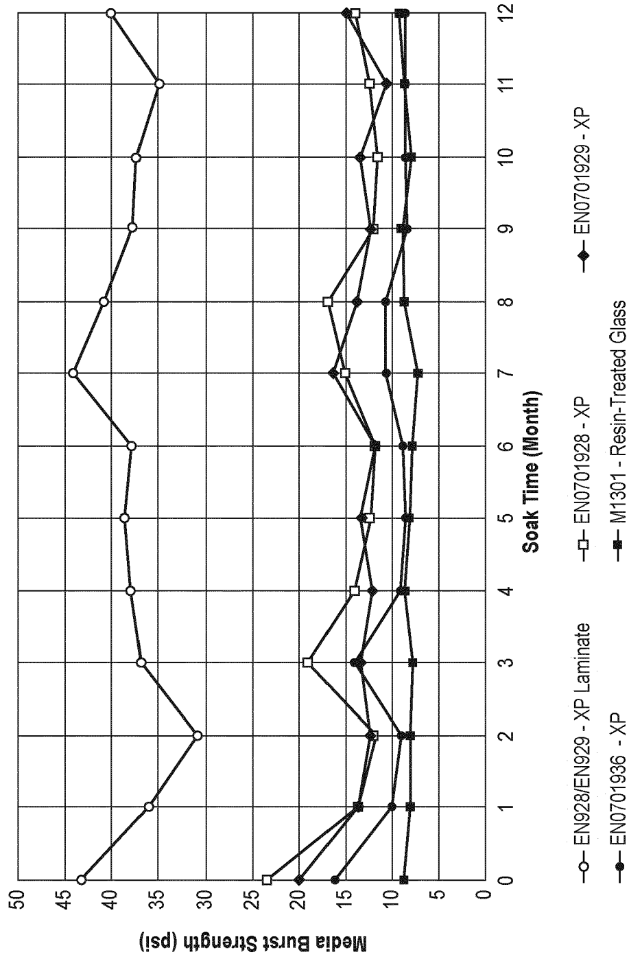
12 Month 150°F Flatsheet Skydrol Soak Compatibility Testing
