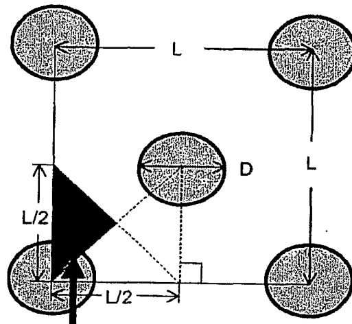
Repeating Geometric Element Modeled by FEMLAB
