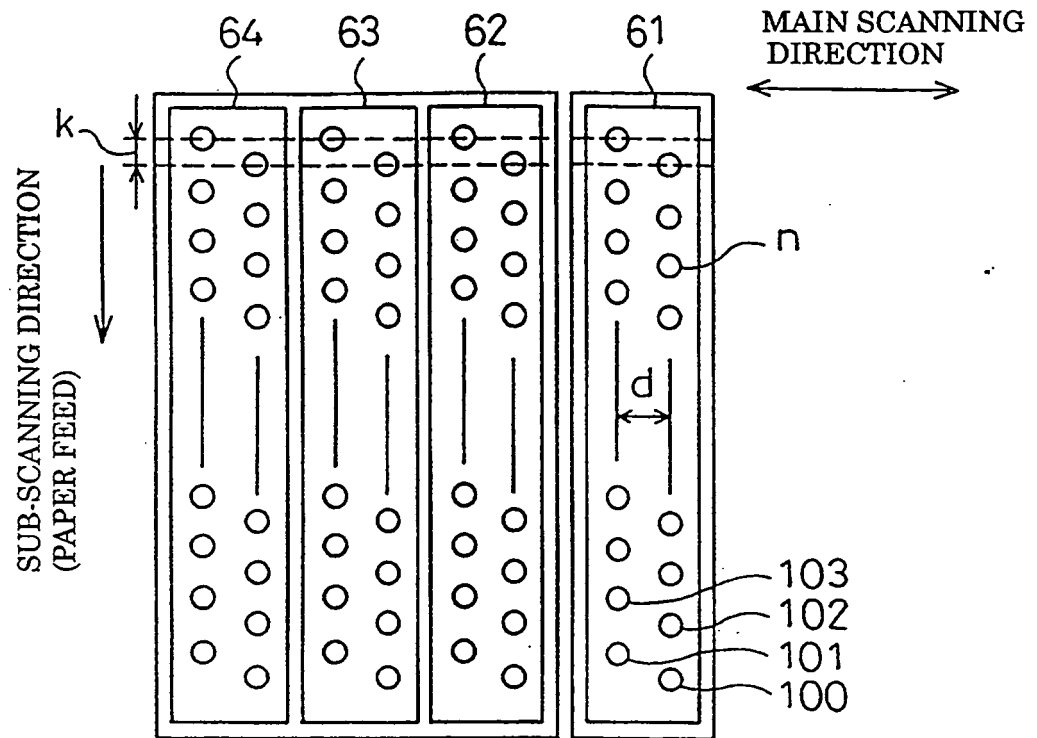
Fig. 5 (B) DOTS FORMED BY ONE NOZZLE ARRAY
