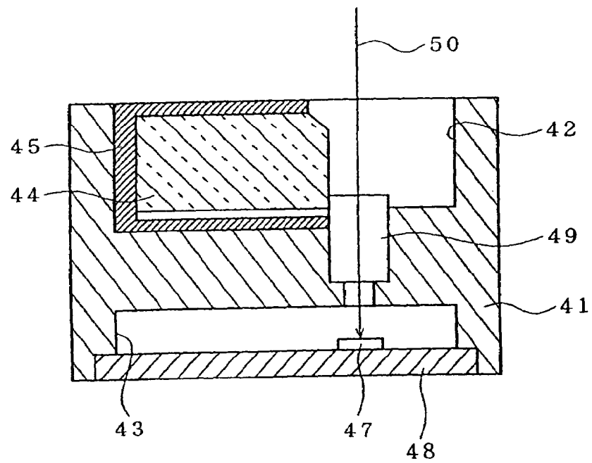
FIG. 12 PRIOR ART
