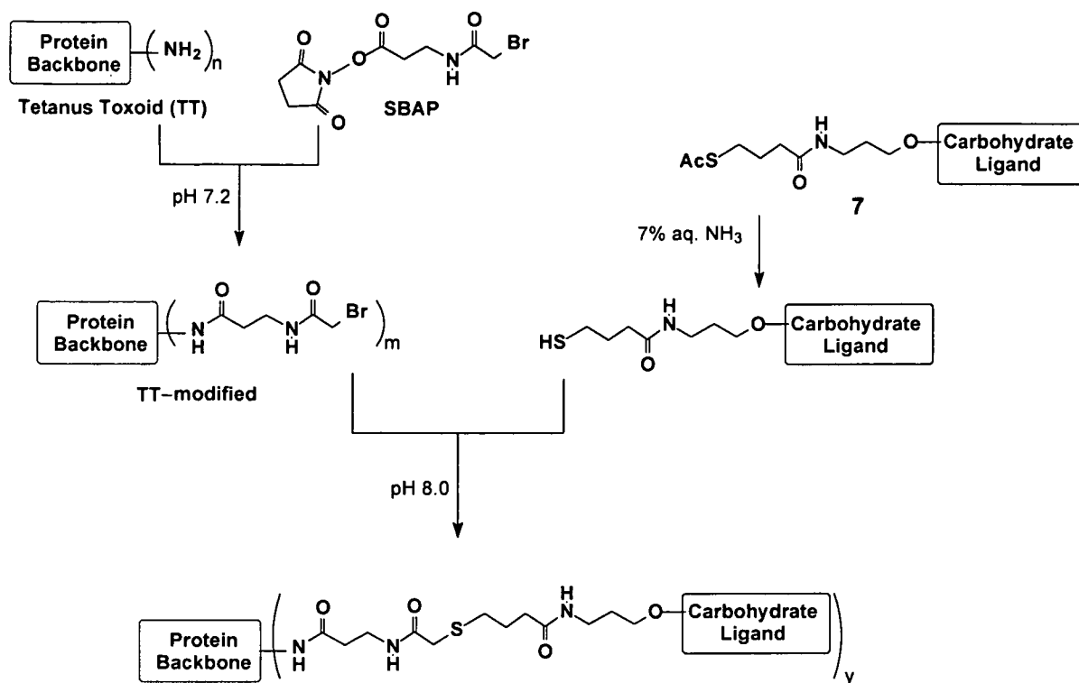
Conjugate of Tetanus Toxoid with Ligand 7 ("TT-9NAc") Scheme 7. Conjugation with Ligand 7.
