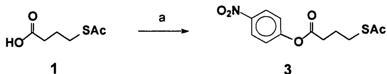
Scheme 2. Synthesis of the linking reagent 3. a: CF 3 COOPnp, Et 3 N.
