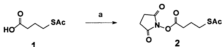
Scheme 1. Synthesis of the linking reagent 2. a: CF 3 COOSu, pyridine.
