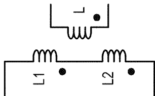
balun 980
