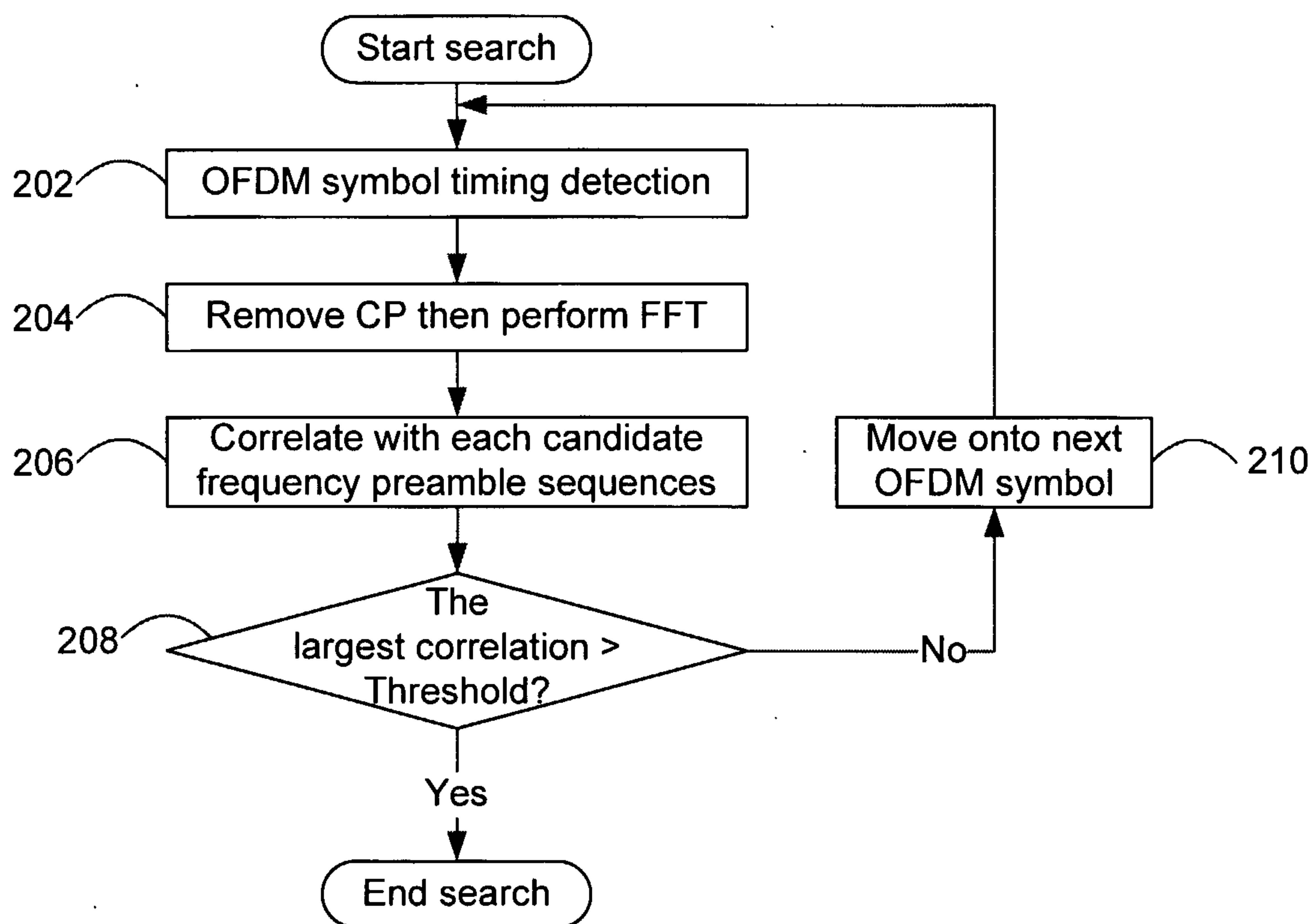
FIG.2 (PRIOR ART)
