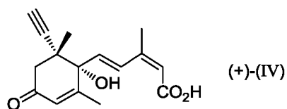
8'-acetylene ABA
