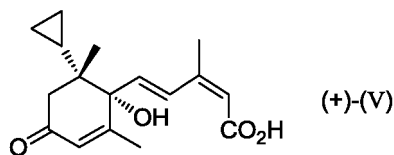
8'-cyclopropyl ABA
