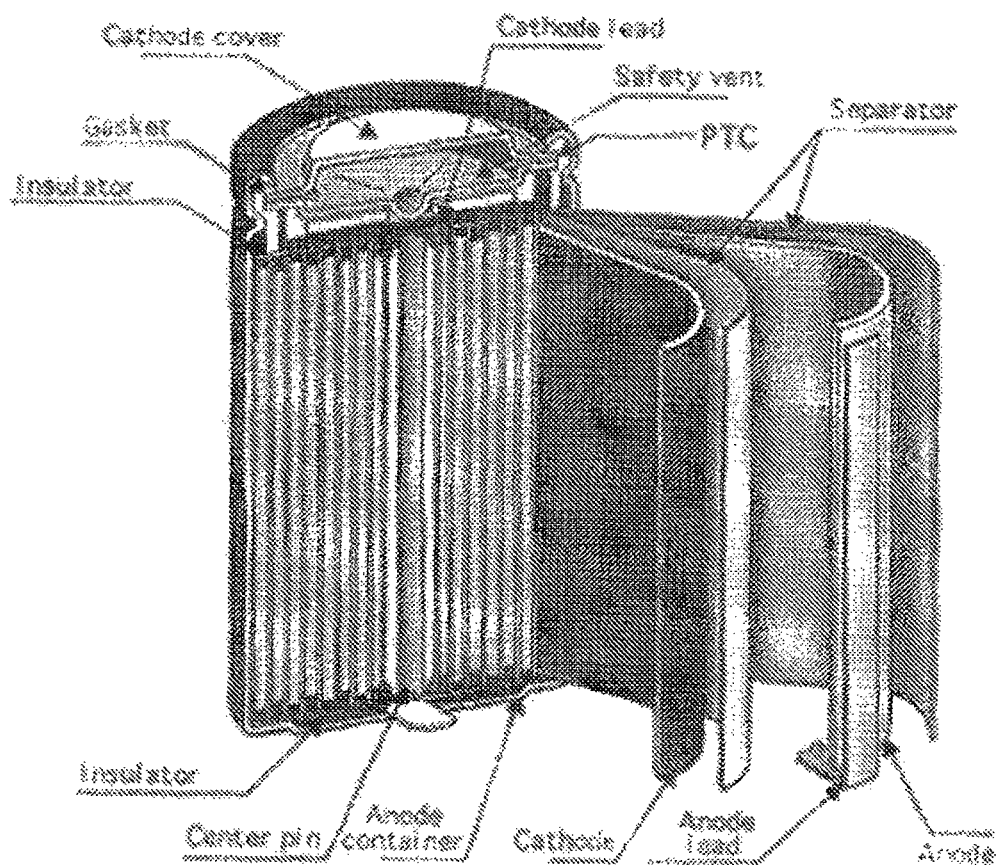
Figure 1—Wound cell
