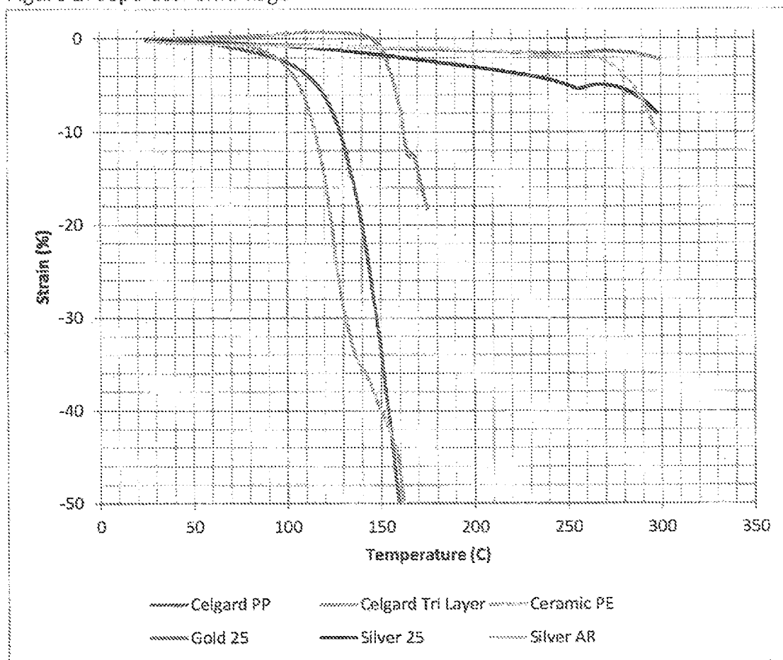
Figure 2: Separator Shrinkage
