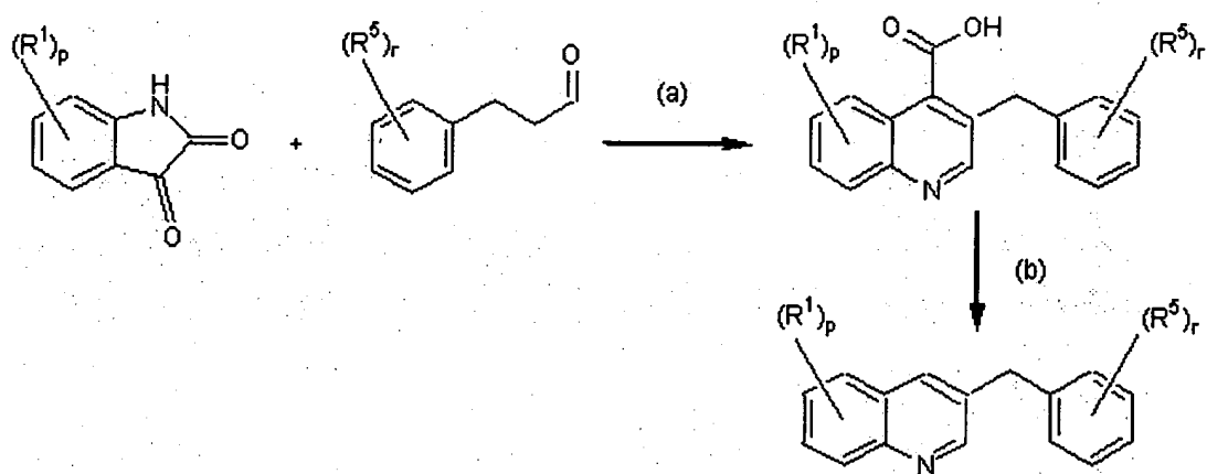
(V-a-2)
