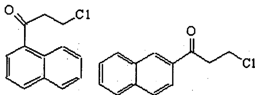
Intermediate 5
