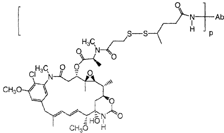
Ab-SPP-DM1
