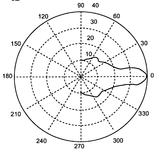
polar_0deg_10000Hz
