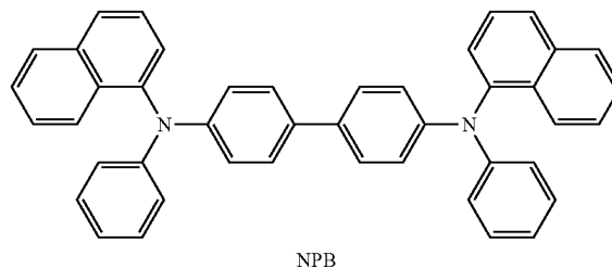
NPB
