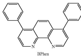
BPhen
