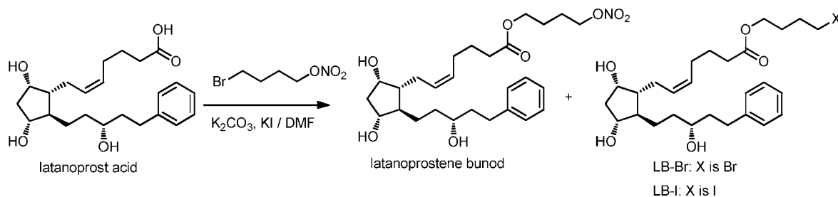
Scheme 1
