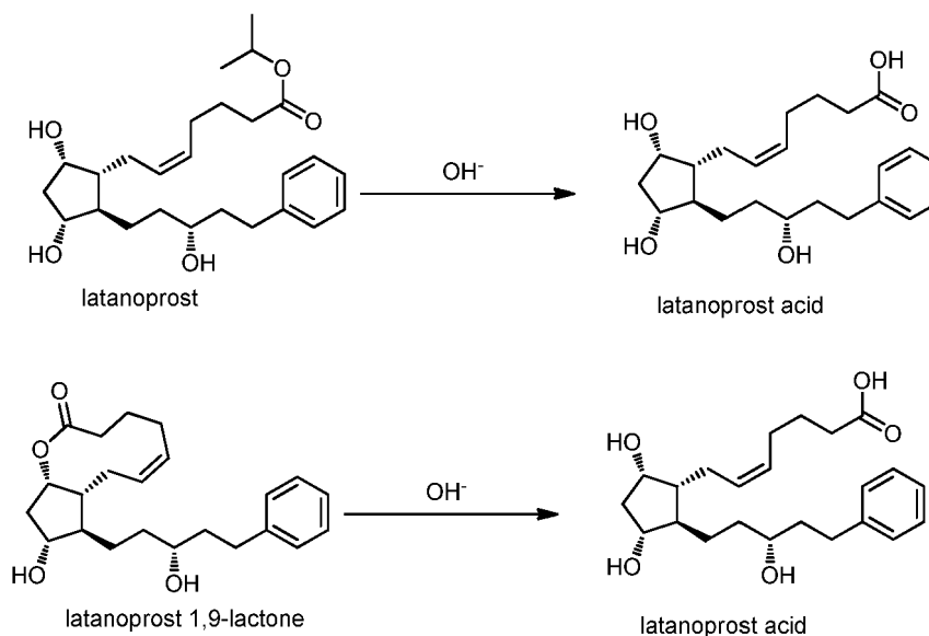
Scheme 3
