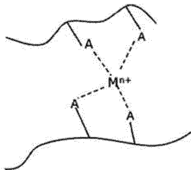
Schematic scheme for reaction (V)
