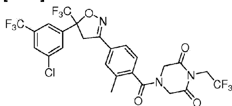
Compound 69
