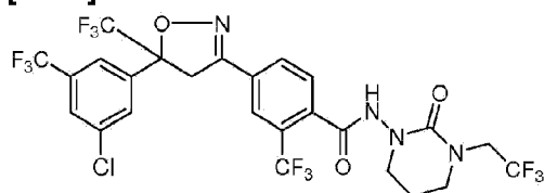
Compound 97
