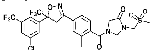
Compound 114
