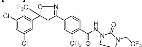
Compound 67
