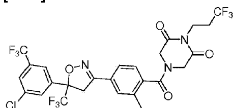
Compound 79
