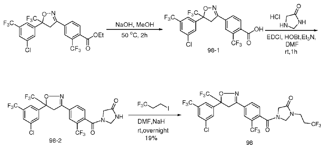
Scheme 12
