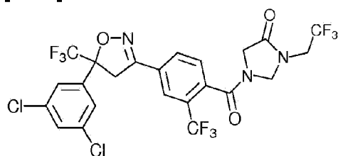
Compound 93
