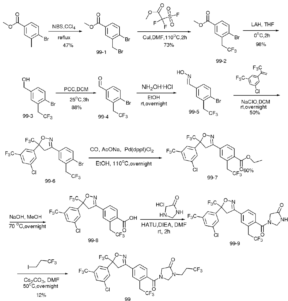
Scheme 13
