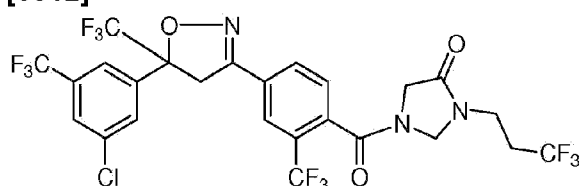
Compound 98
