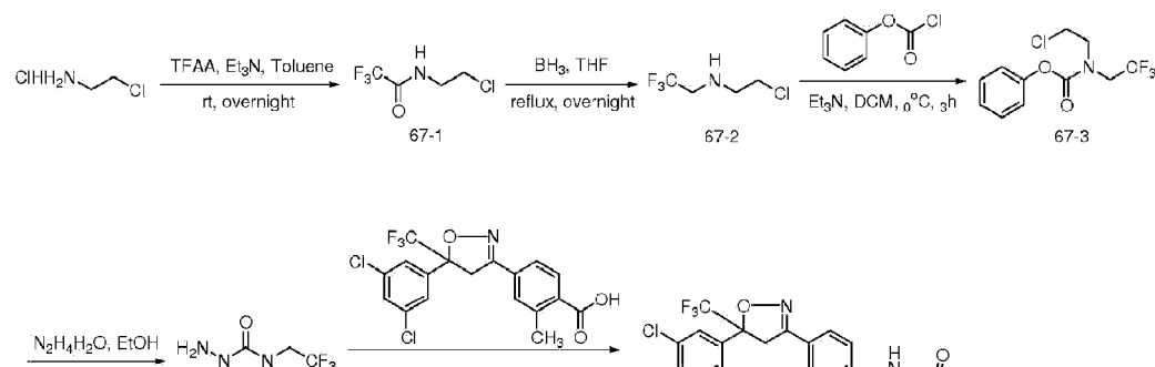
Scheme 3
