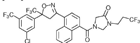
Compound 112
