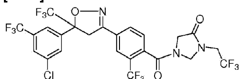
Compound 96
