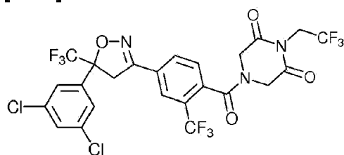
Compound 92
