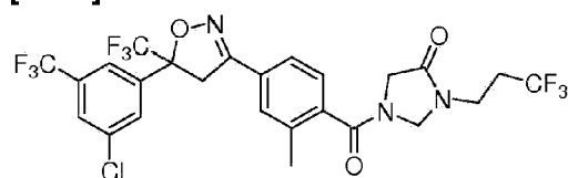
Compound 80
