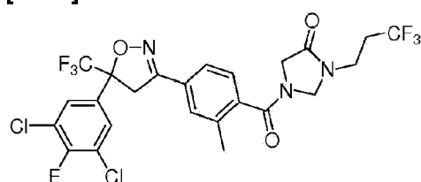
Compound 115
