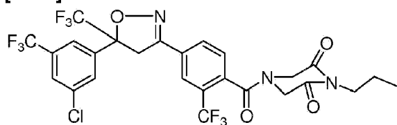
Compound 95
