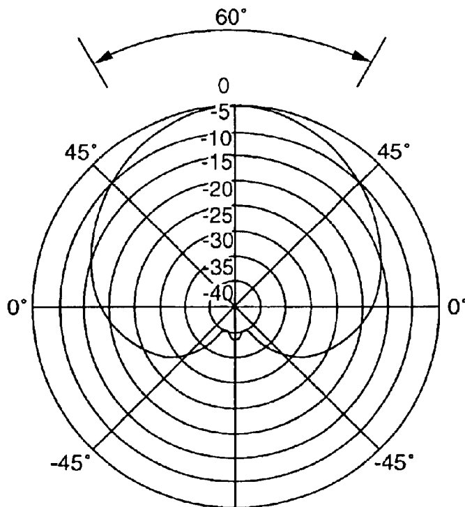
FIG. 7 POWER RELATIVE TO PEAK POWER (dB)
